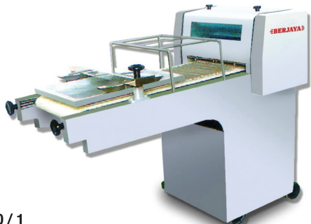
Dough Moulder Capacity(Pcs/time): 1000 - 3000 Working Wide(mm): 390 Voltage/Phase(V/Ph): 220 - 240 / 1
